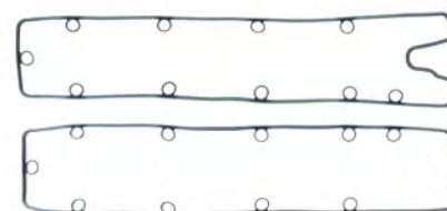
Peugeot 206, 406 EW10J4 Rocker Cover: RC3304 In. Rocker Cover: RC3305 Exh.
